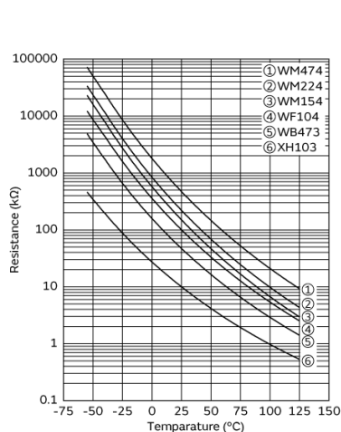
Resistance-Temperature Characteristics
